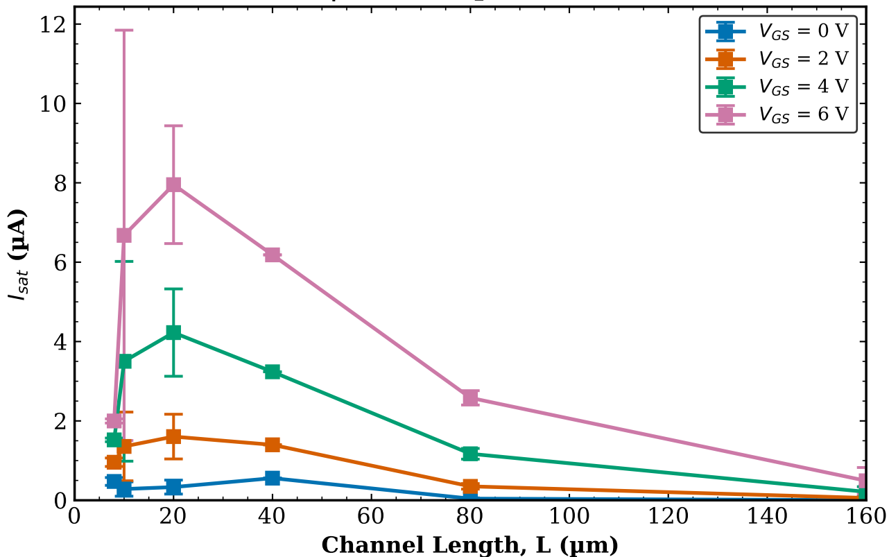
TFT3 Combined (Tr. 1 & 2) I_{sat} vs L | W = 10 \mu\text{m} (mean \pm std)
